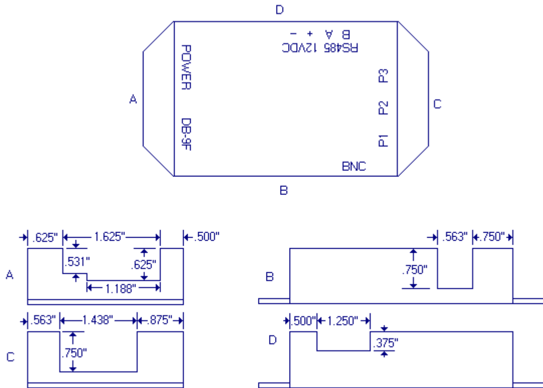
HOME AUTOMATION GATEWAY ENCLOSURE (NOT TO SCALE) NOTE: Dimensions are not exact. Cut openings undersize and file to fit. POLYCASE LP-31F
